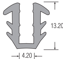
PVC channel
